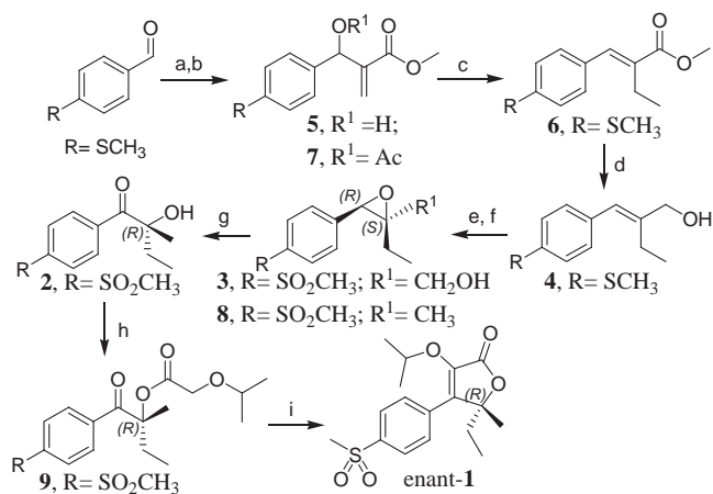
Scheme 2. Synthesis of enantiomeric 1 . Reagents and conditions: a. Methyl acrylate, DABCO, ultrasound, 48 h, 79%; b. AcCl, Et 3 N, DMAP, CH 2 Cl 2 , 0 °C, 12 h, 88%; c. CH 3 Li, CuI, -20 to -40 °C, 10 h, 60%; d. DIBAL-H, CH 2 Cl 2 , -78 °C, 2 h, 89%; e. (-)-DIPT, Ti(O i Pr) 4 , TBHP, CH 2 Cl 2 , -40 to -20 °C, 70%, 76% ee f. (i) MsCl, Et 3 N, CH 2 Cl 2 , 0 °C, 10 min; (ii) LiAlH 4 , THF, 0 °C, 30 min, 70% (for two steps); g. 20 mol % Pd(OAc) 2 , bathocuproine (20 mol %), H 2 O, O 2 , 100 °C, 30 h, 55%; h. DPC, DMAP, 2-isopropoxy acetic acid, DCE, 70%; i. CF 3 CO 2 i Pr, DBU, CH 3 CN, reflux, 10 h, 85%.
